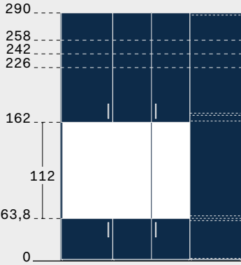
Nicchia maxi Maxi recess
